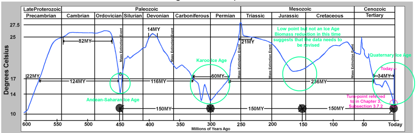
Average Global Temperature
