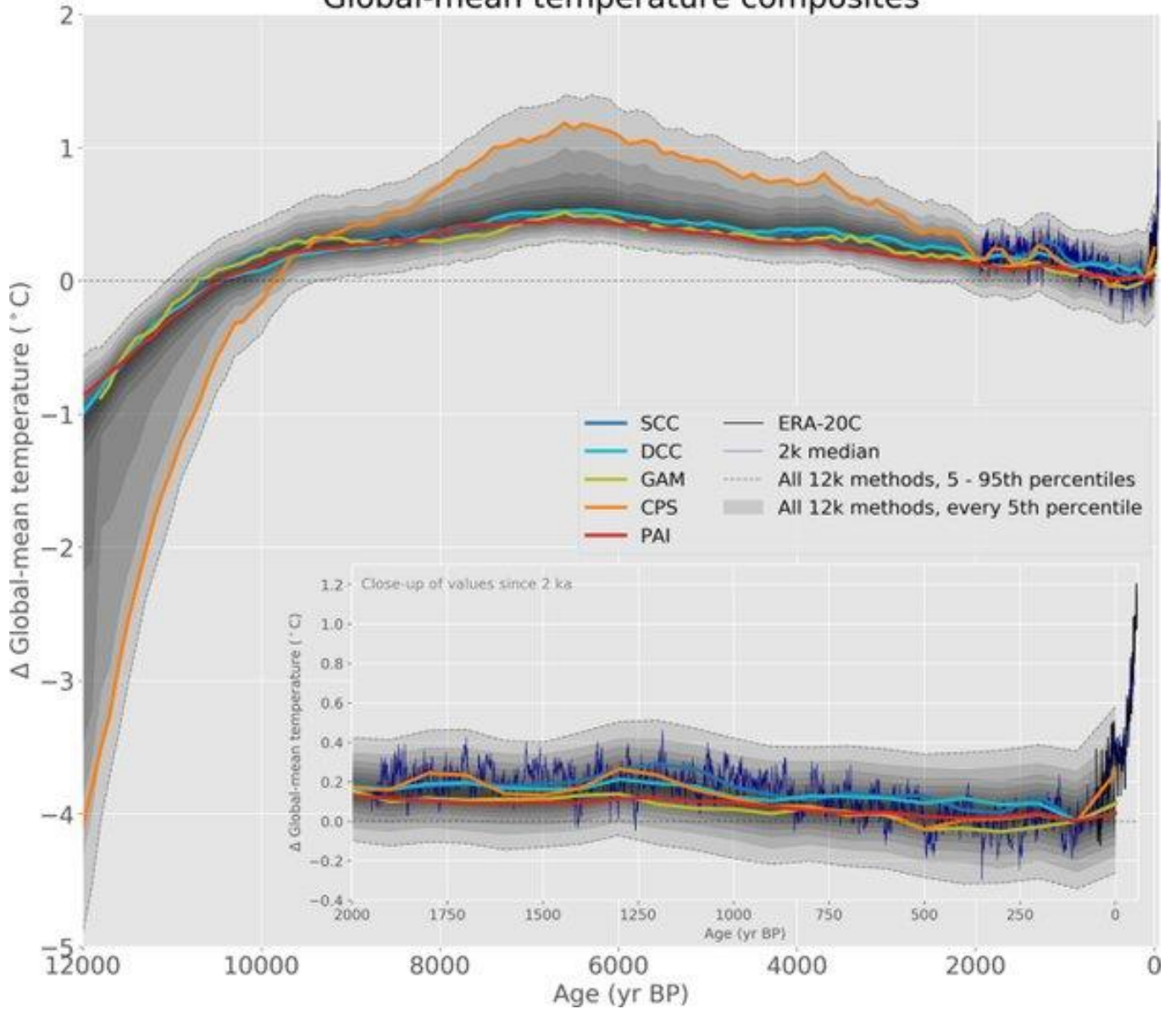
Global-mean temperature composites
