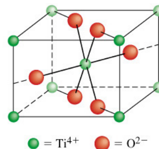
(c) Unit cell of TiO_2 , the rutile structure
