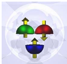
Plasma model; green for matter, red for antimatter, and dark blue for dark matter.
