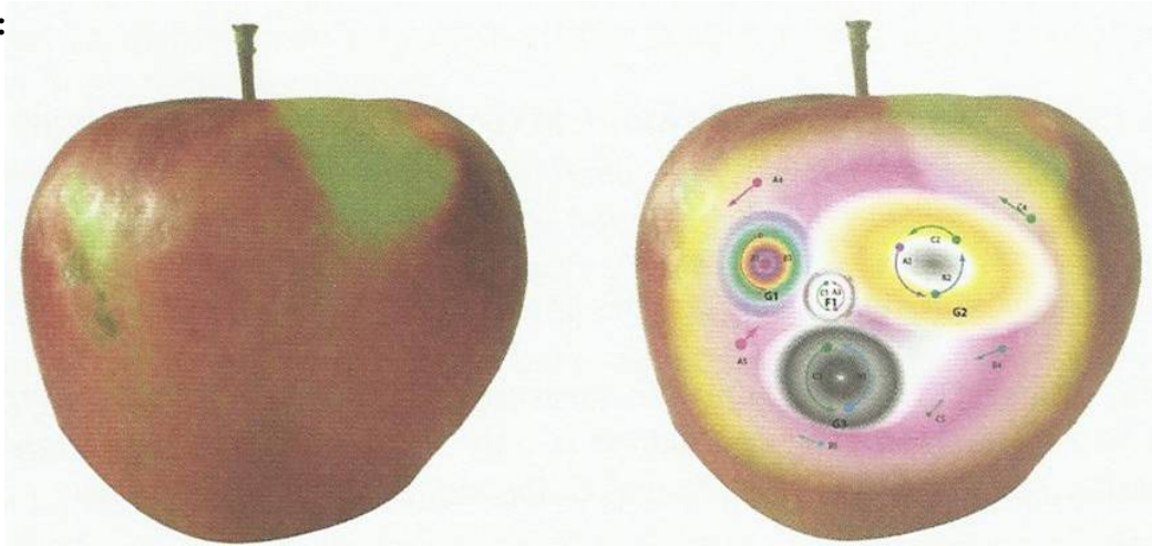
Newton's apple has different types of plasma of magnetic fields and plasma matter magnetic fields.
