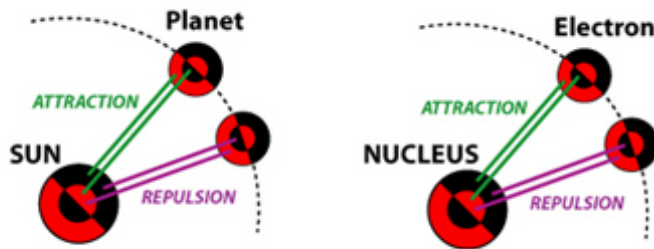
Simplified image as Double Solid Magnets These effects happen however on loosely-bounded molecular level.
