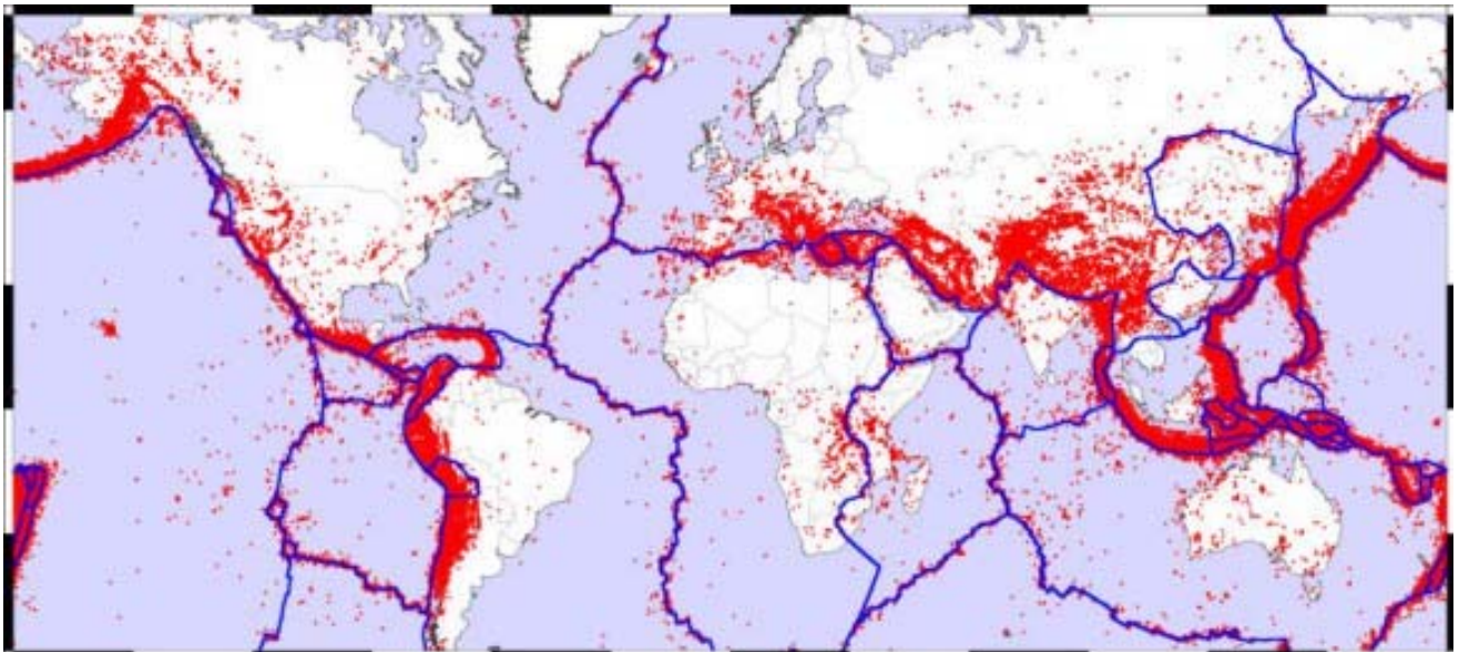
Map of the Earth showing the relation between fault lines (blue) and zones of volcanic activity (red). Credit: zmescience.com
