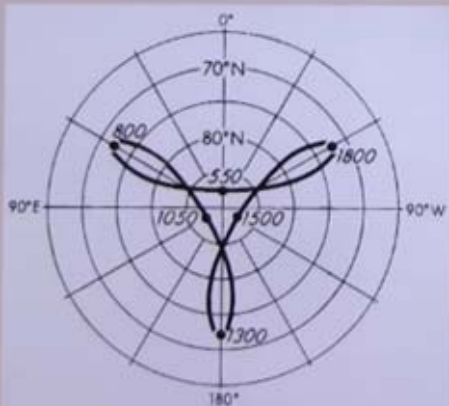
Fig. 1 Model of quasi-hypocycloid motion of the geomagnetic dipole axis during historic times. Numbers on the curve represent dates in yr AD (after N. Kawai and K. Hirooka').
